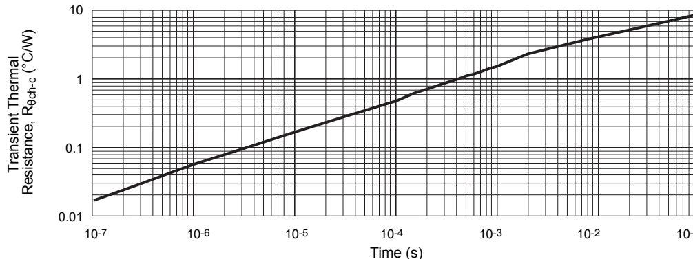
Transient Thermal Resistance Curve
